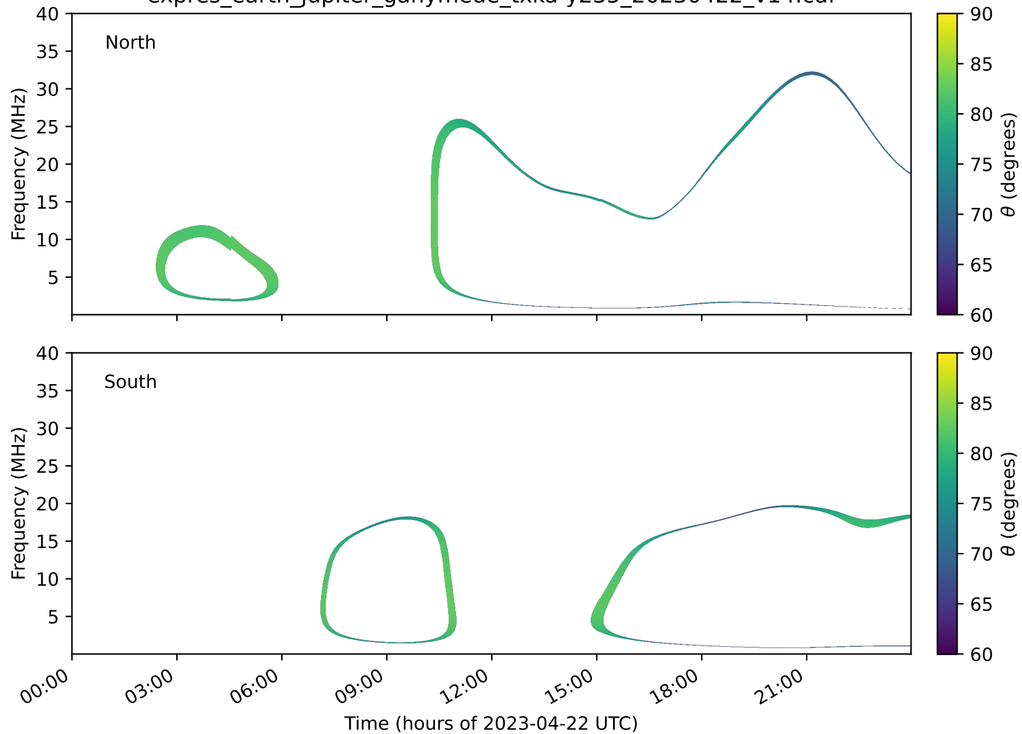
expres_earth_jupiter_ganymede_txka-y235_20230422_v14.cdf
