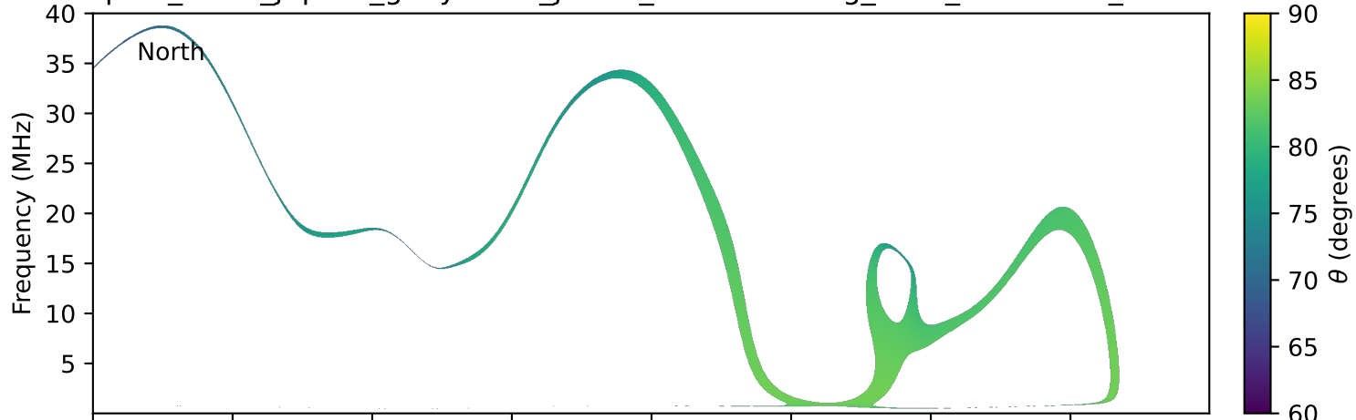
expres_earth_jupiter_ganymede_jrm33_lossc-wid1deg_3kev_20230425_v11.cdf
