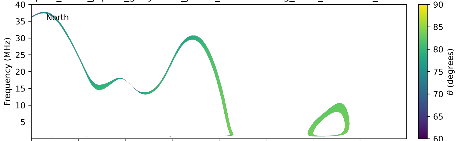
expres_earth_jupiter_ganymede_jrm33_lossc-wid1deg_3kev_20230418_v11.cdf
