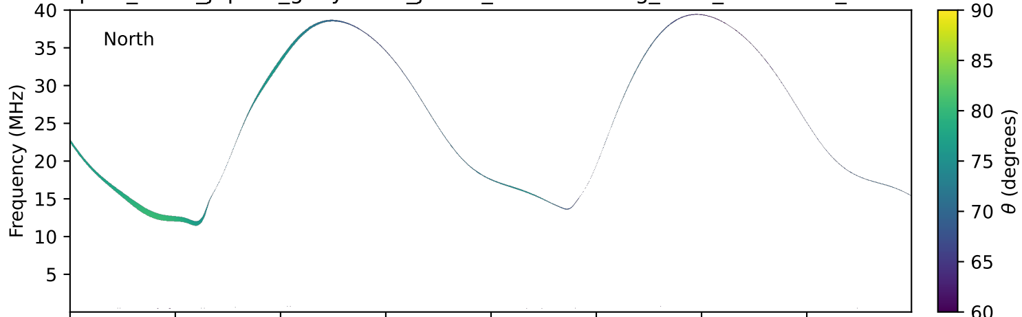
expres_earth_jupiter_ganymede_jrm09_lossc-wid1deg_3kev_20230430_v11.cdf
