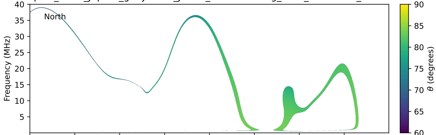
expres_earth_jupiter_ganymede_jrm09_lossc-wid1deg_3kev_20230425_v11.cdf
