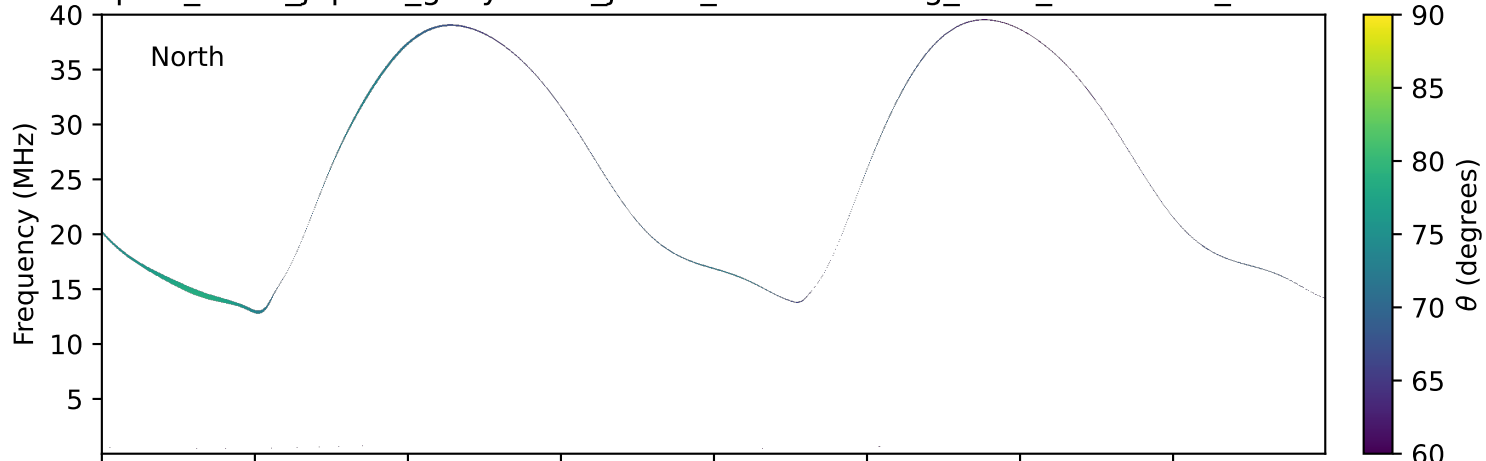
expres_earth_jupiter_ganymede_jrm09_lossc-wid1deg_3kev_20230423_v11.cdf
