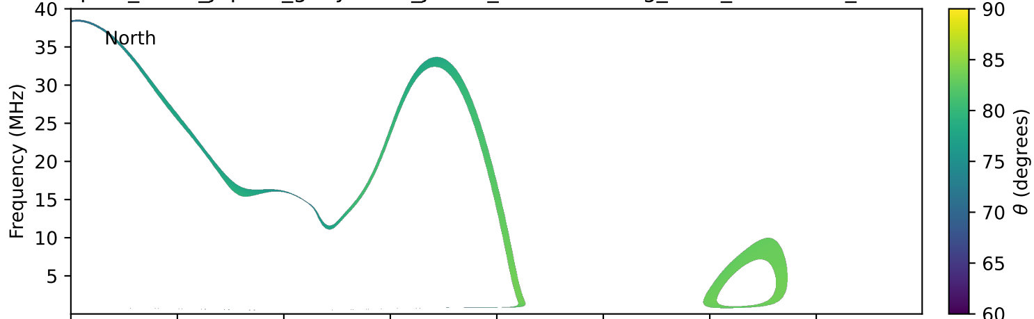
expres_earth_jupiter_ganymede_jrm09_lossc-wid1deg_3kev_20230418_v11.cdf
