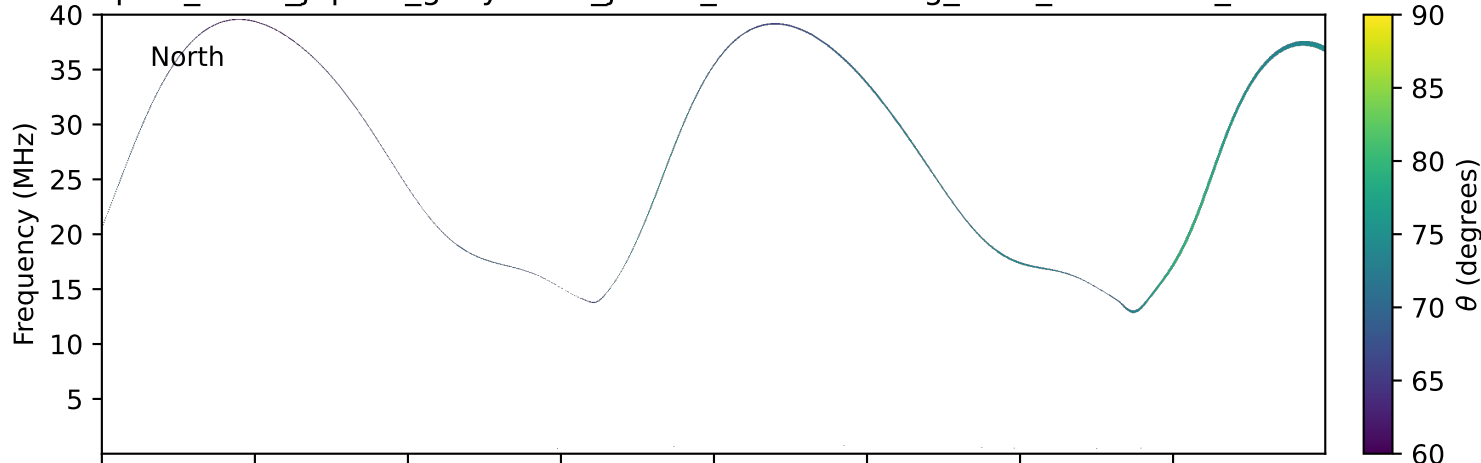
expres_earth_jupiter_ganymede_jrm09_lossc-wid1deg_3kev_20230410_v11.cdf
