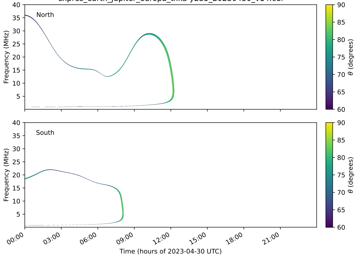
expres_earth_jupiter_europa_txka-y235_20230430_v14.cdf
