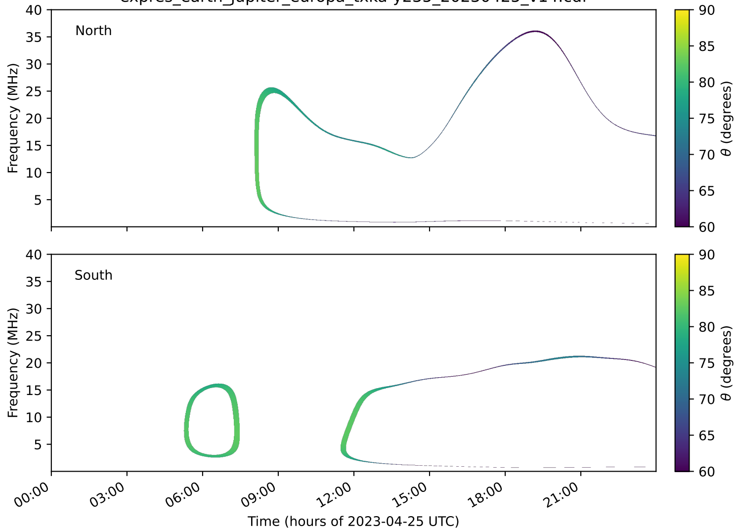
expres_earth_jupiter_europa_txka-y235_20230425_v14.cdf
