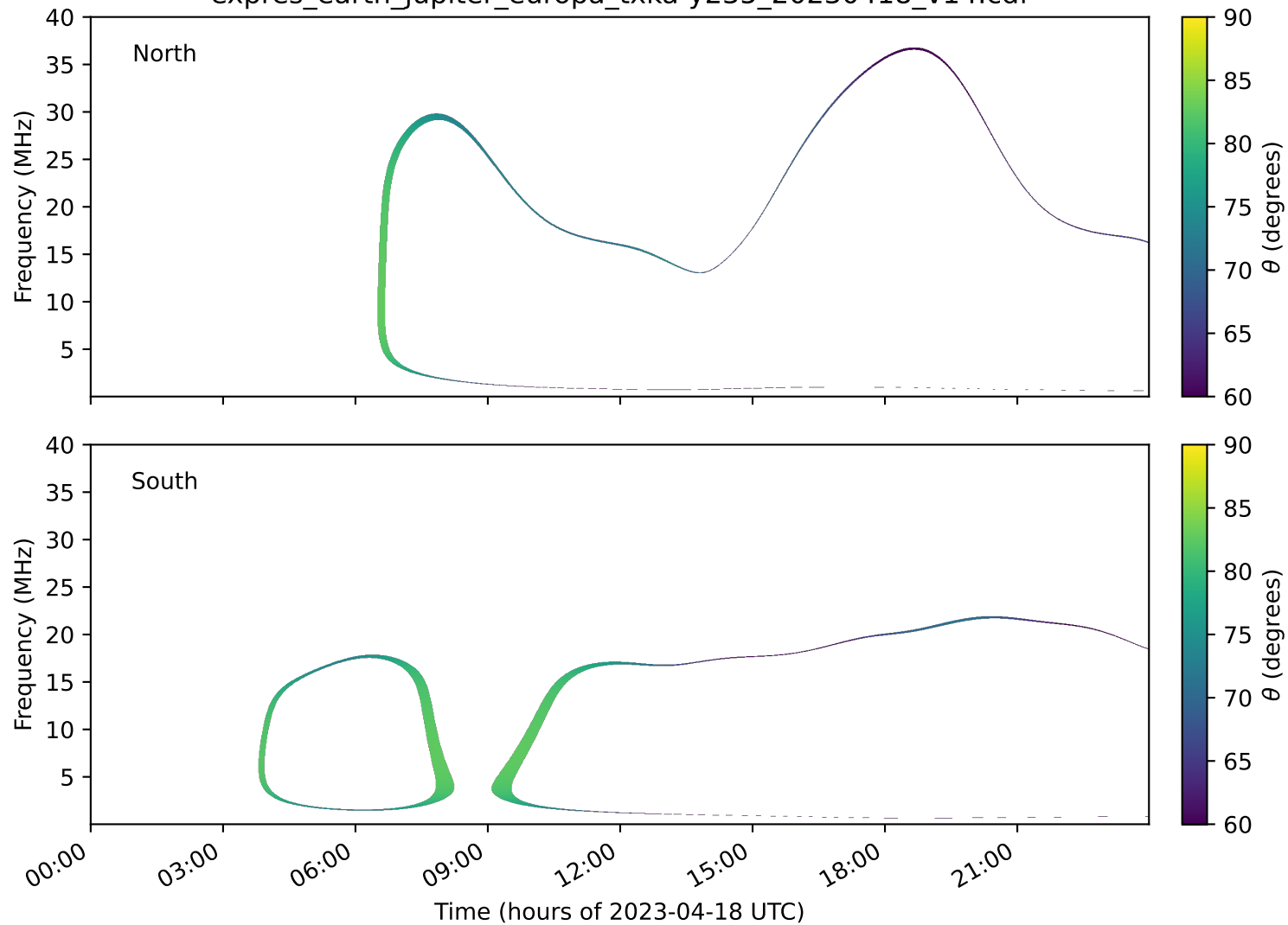
expres_earth_jupiter_europa_txka-y235_20230418_v14.cdf
