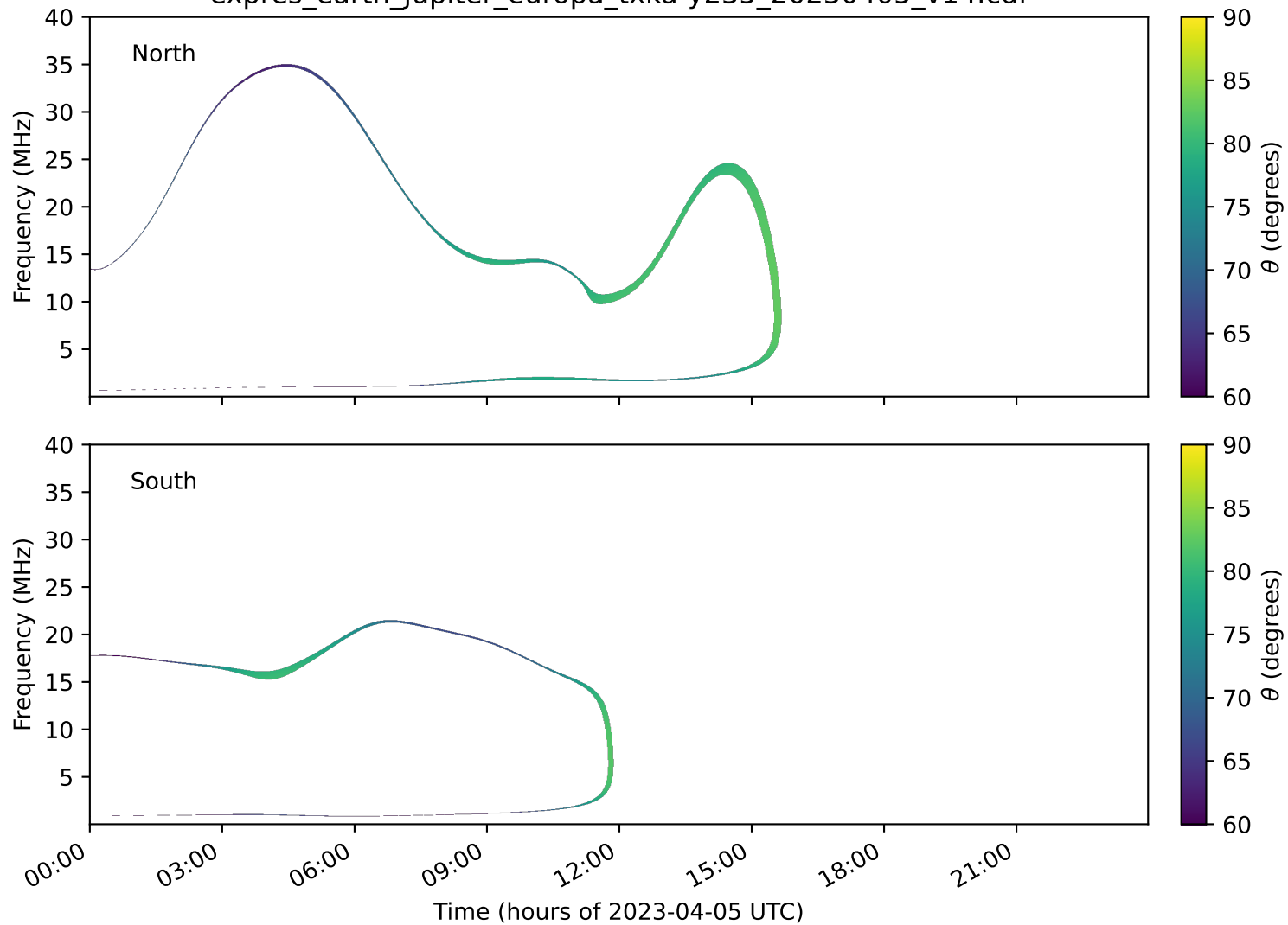
expres_earth_jupiter_europa_txka-y235_20230405_v14.cdf
