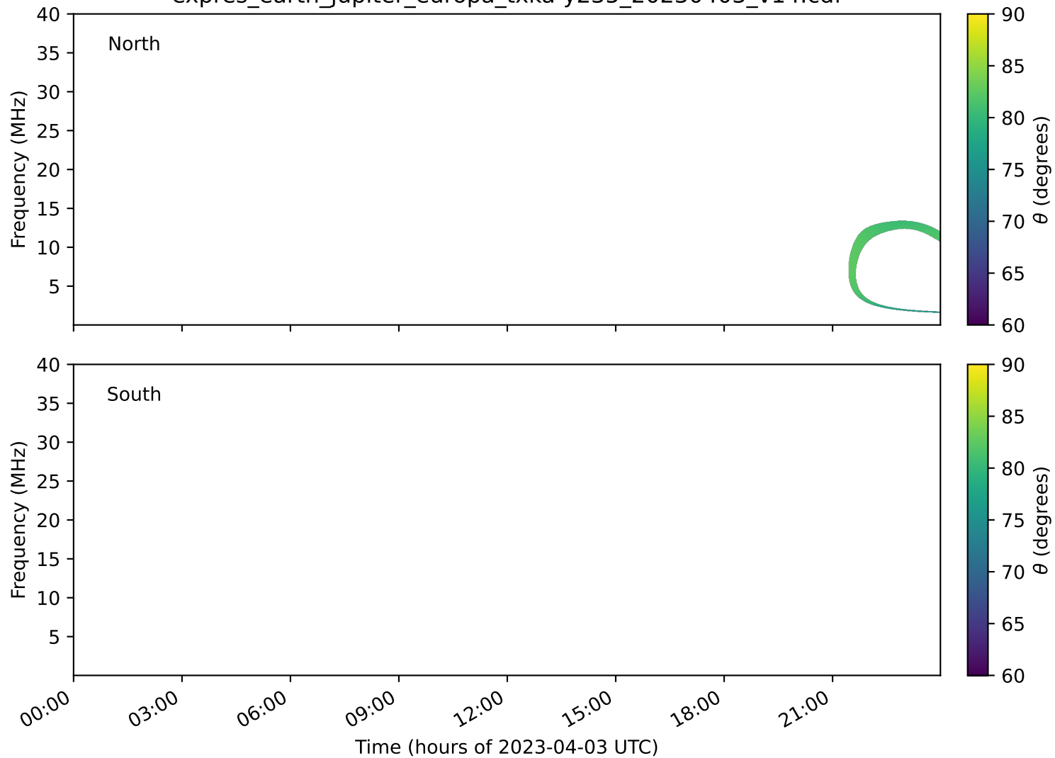
expres_earth_jupiter_europa_txka-y235_20230403_v14.cdf
