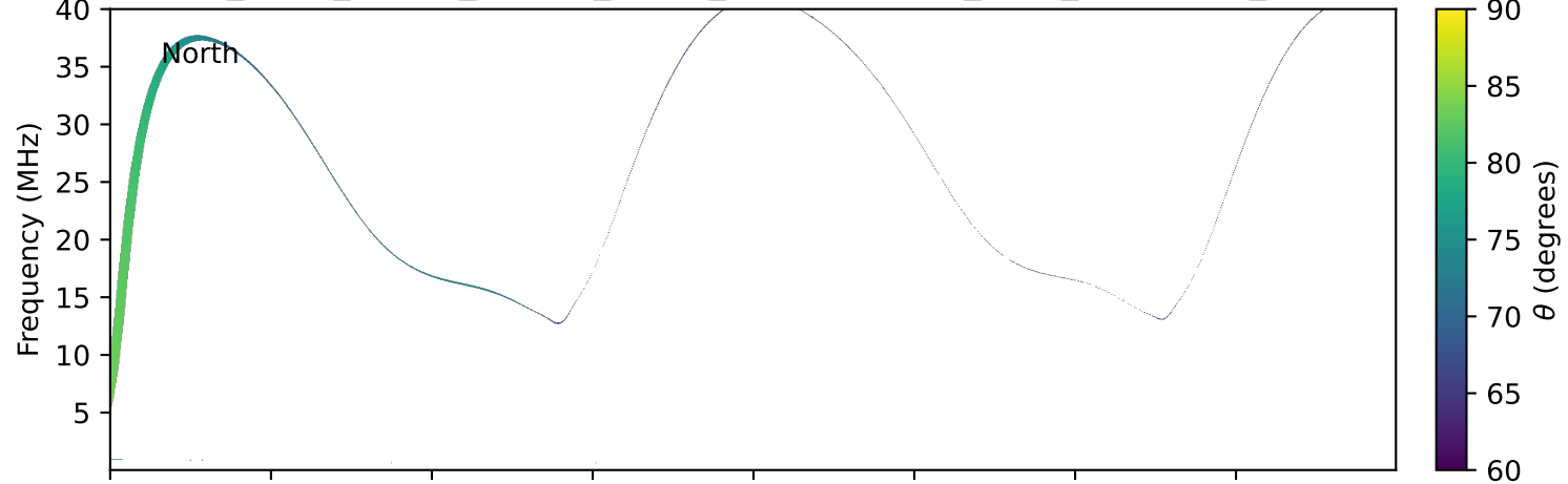
expres_earth_jupiter_europa_jrm09_lossc-wid1deg_3kev_20230429_v11.cdf
