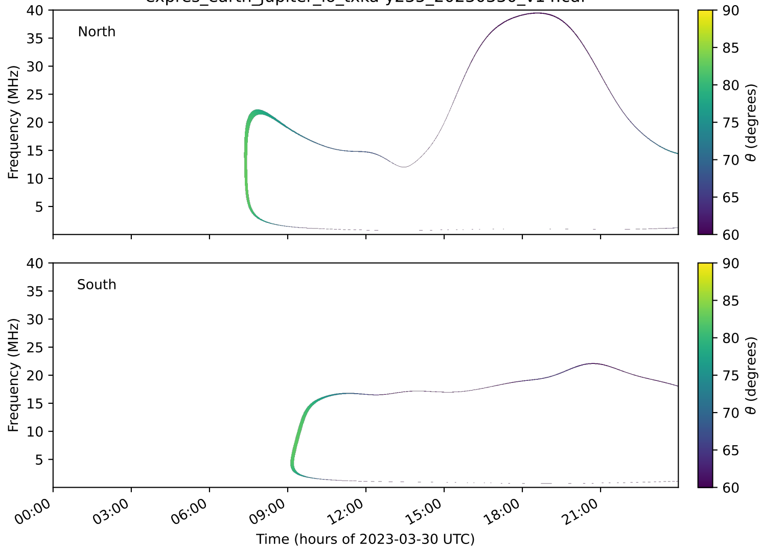
expres_earth_jupiter_io_txka-y235_20230330_v14.cdf
