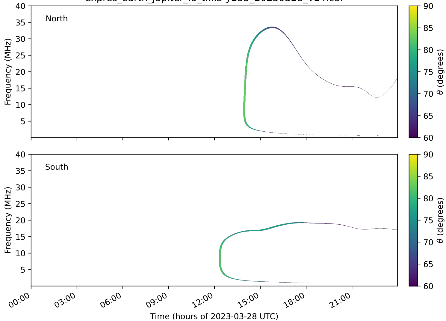
expres_earth_jupiter_io_txka-y235_20230328_v14.cdf
