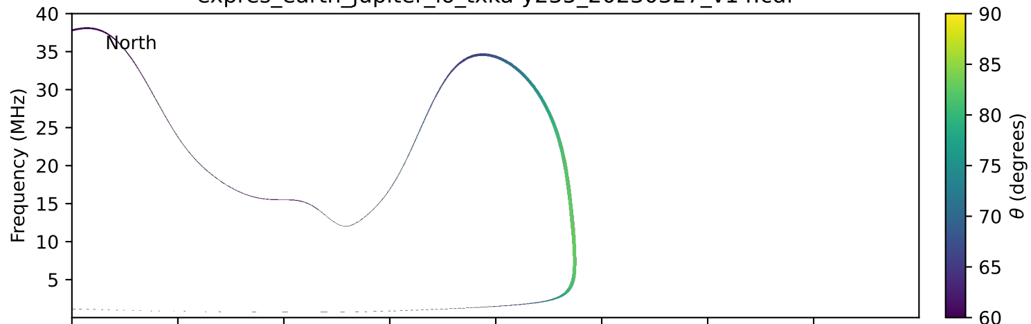
expres_earth_jupiter_io_txka-y235_20230327_v14.cdf
