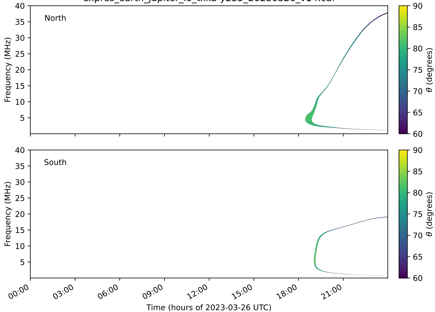
expres_earth_jupiter_io_txka-y235_20230326_v14.cdf
