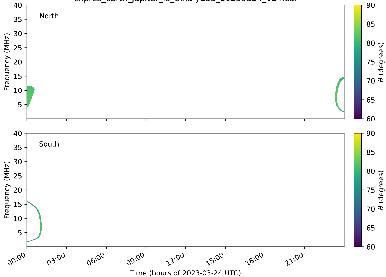
expres_earth_jupiter_io_txka-y235_20230324_v14.cdf
