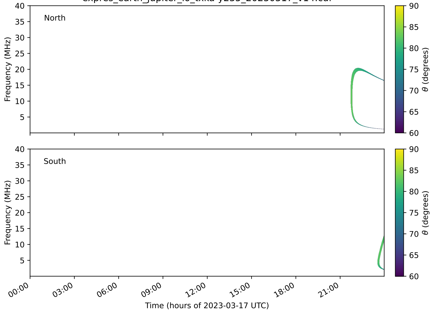
expres_earth_jupiter_io_txka-y235_20230317_v14.cdf
