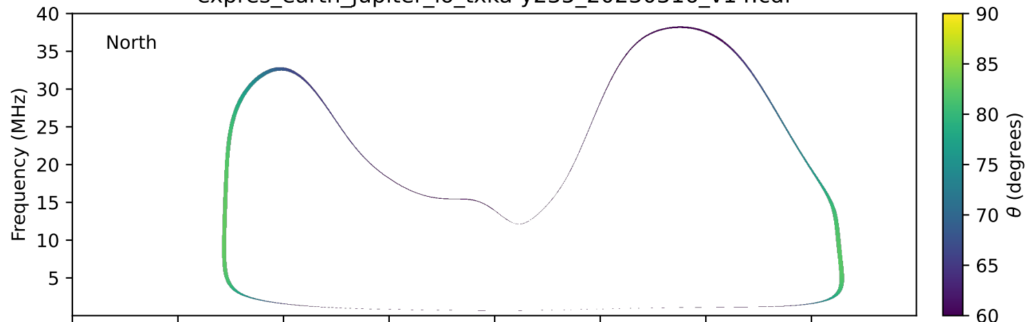
expres_earth_jupiter_io_txka-y235_20230316_v14.cdf
