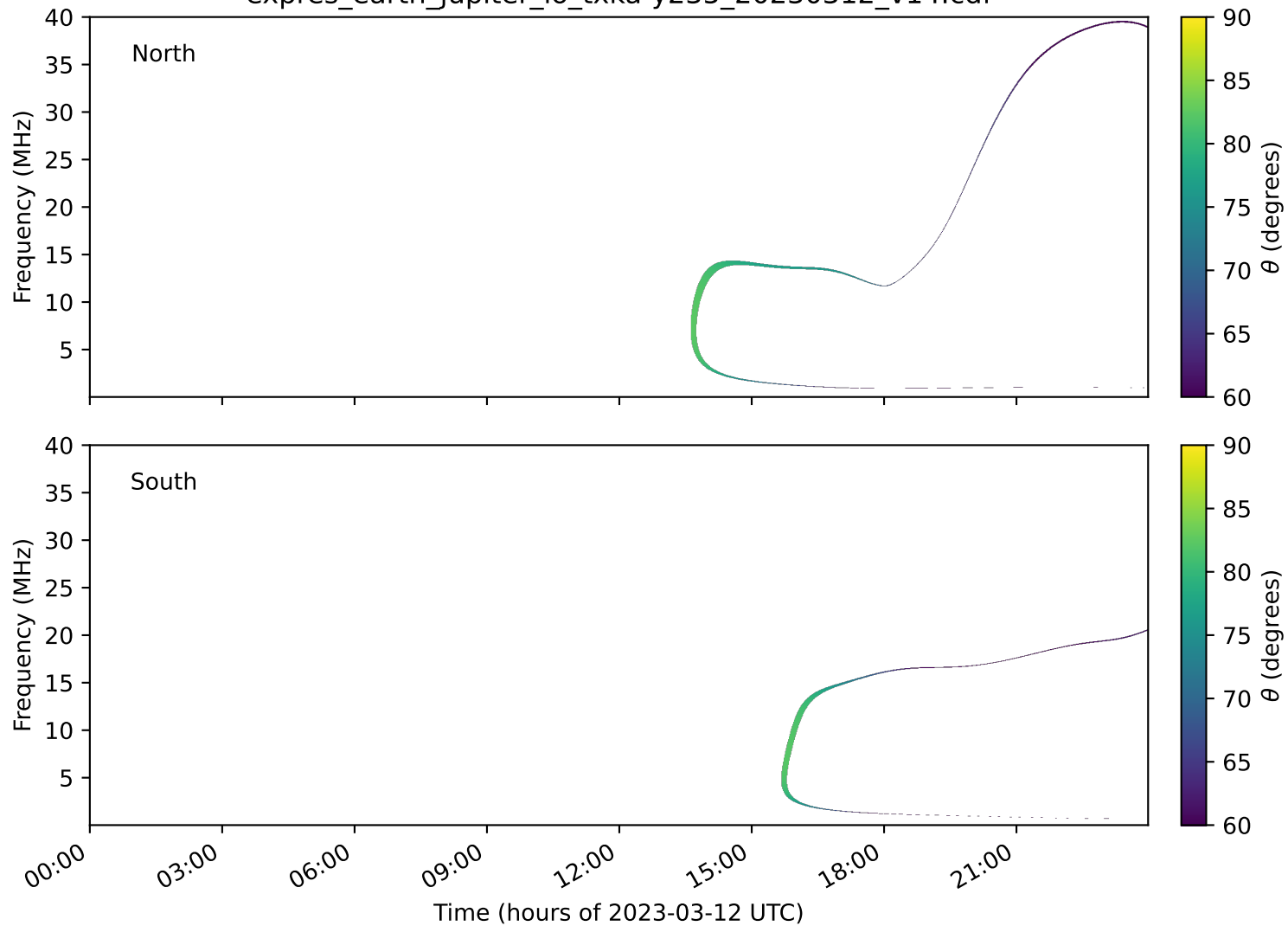
expres_earth_jupiter_io_txka-y235_20230312_v14.cdf
