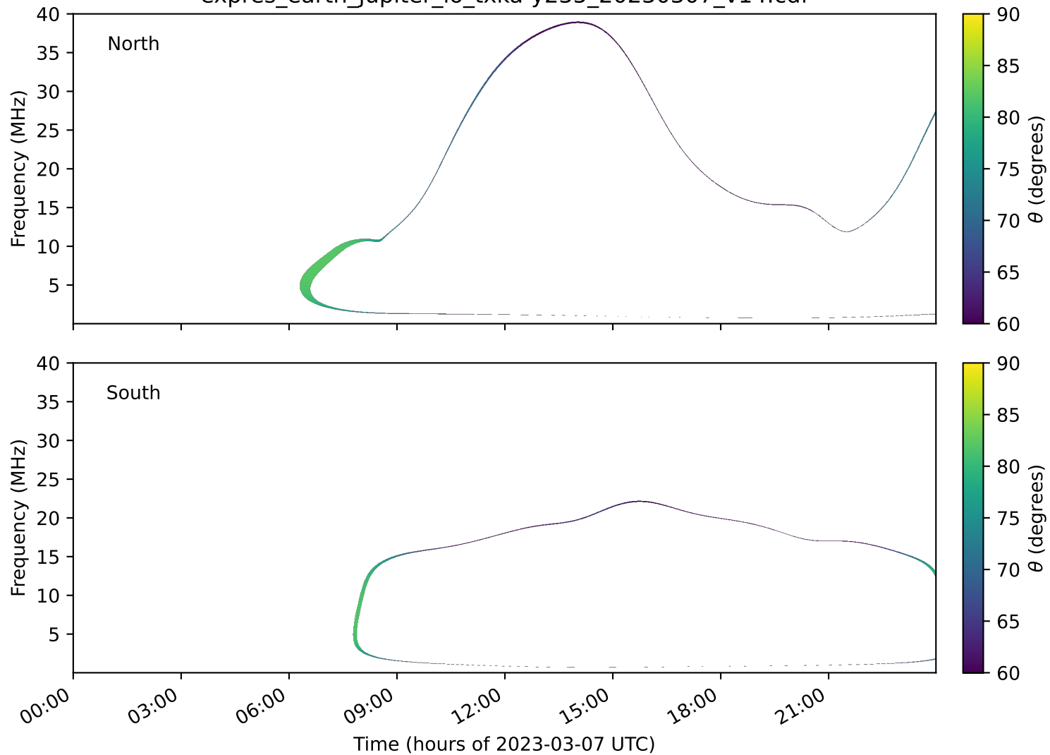
expres_earth_jupiter_io_txka-y235_20230307_v14.cdf
