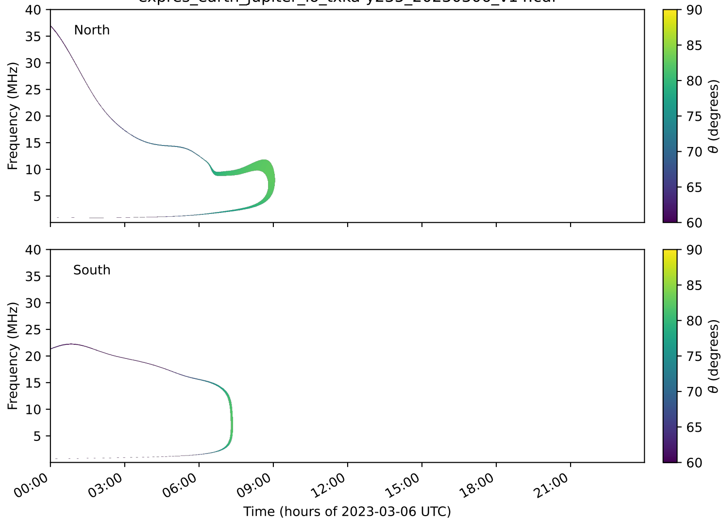
expres_earth_jupiter_io_txka-y235_20230306_v14.cdf
