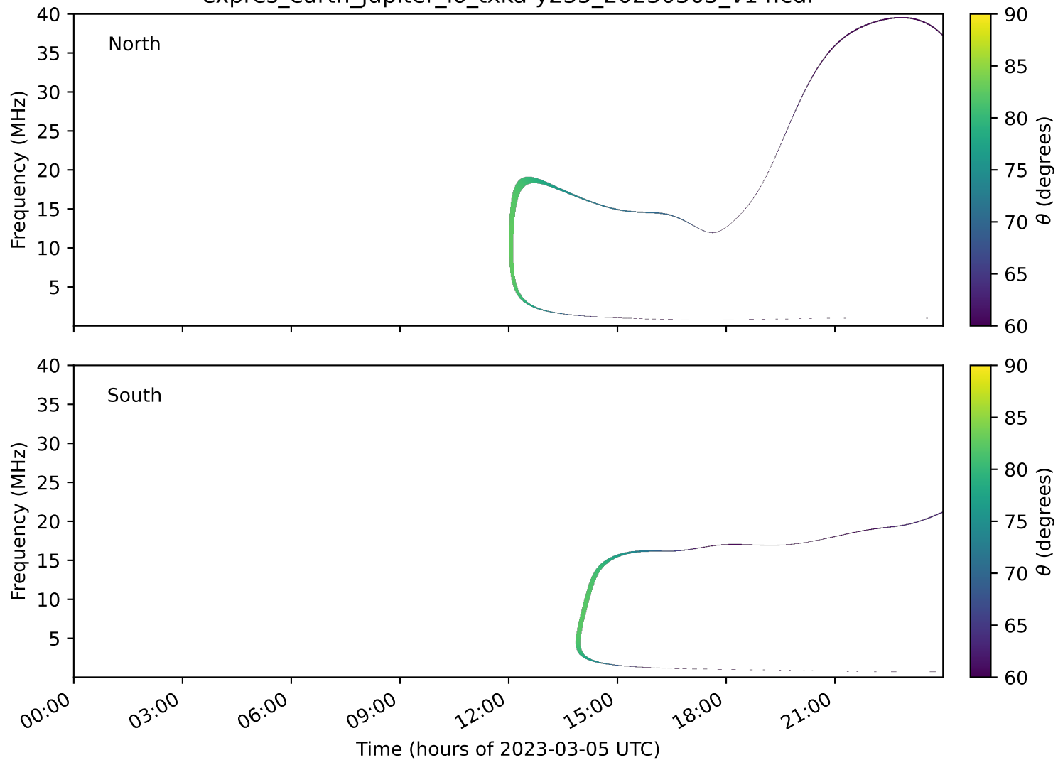
expres_earth_jupiter_io_txka-y235_20230305_v14.cdf
