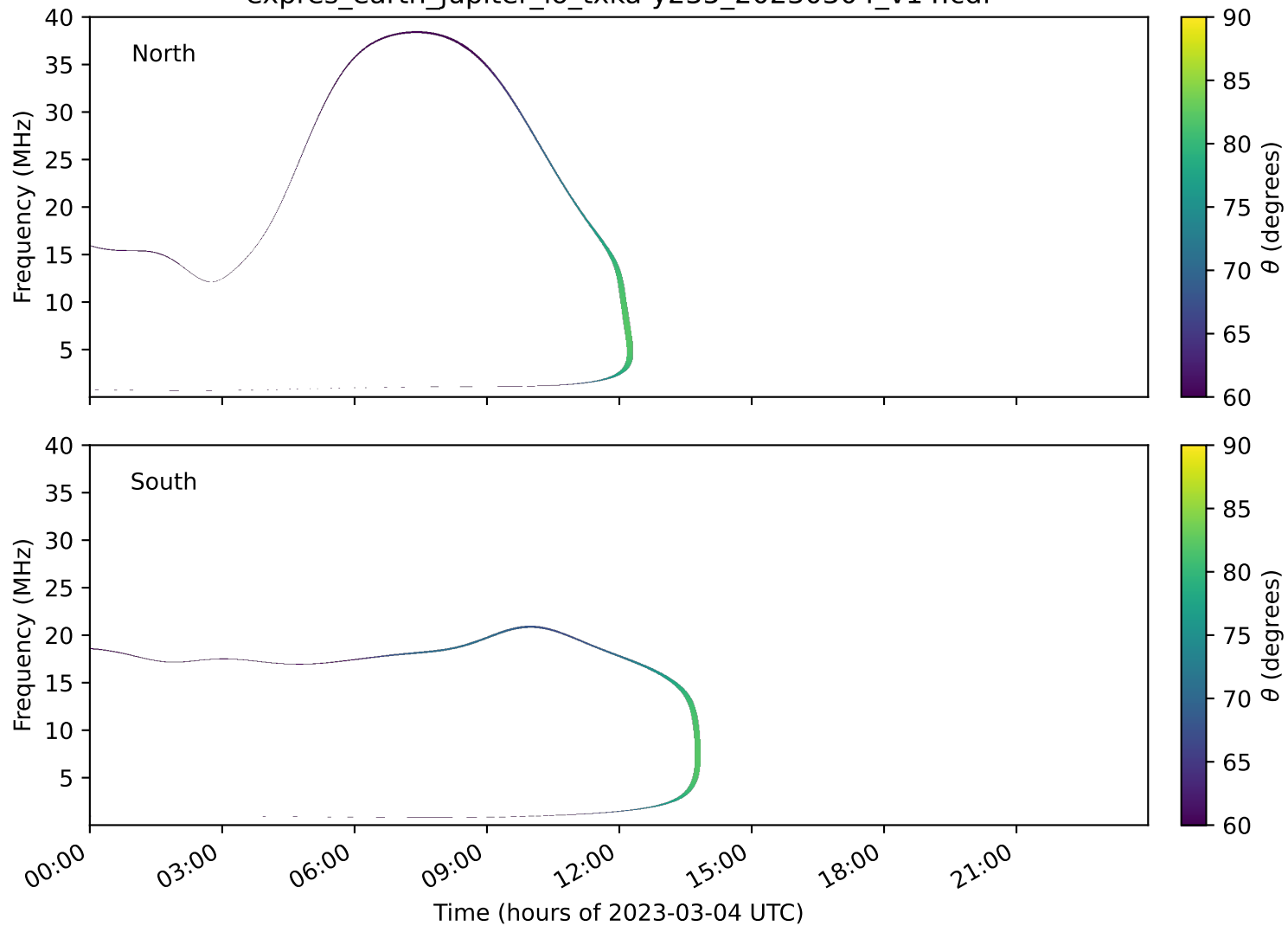
expres_earth_jupiter_io_txka-y235_20230304_v14.cdf
