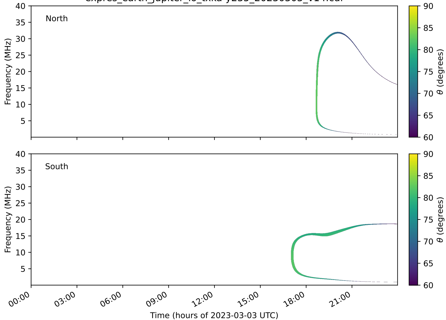
expres_earth_jupiter_io_txka-y235_20230303_v14.cdf
