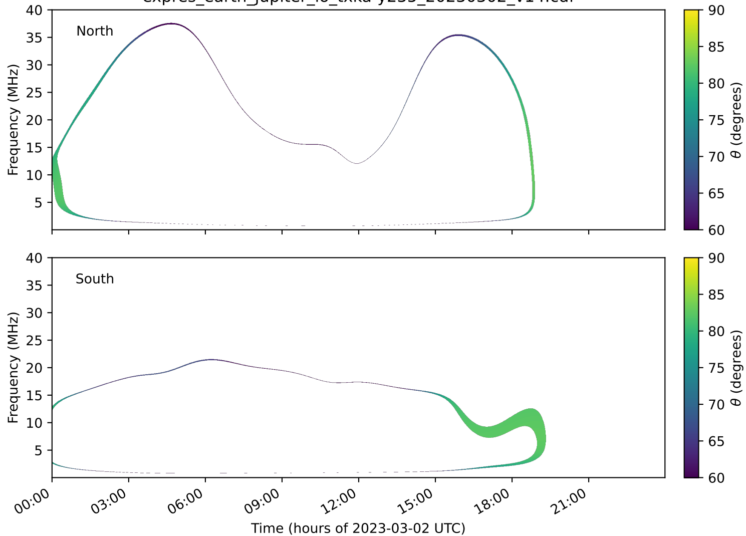
expres_earth_jupiter_io_txka-y235_20230302_v14.cdf
