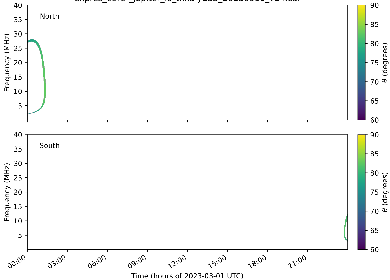
expres_earth_jupiter_io_txka-y235_20230301_v14.cdf
