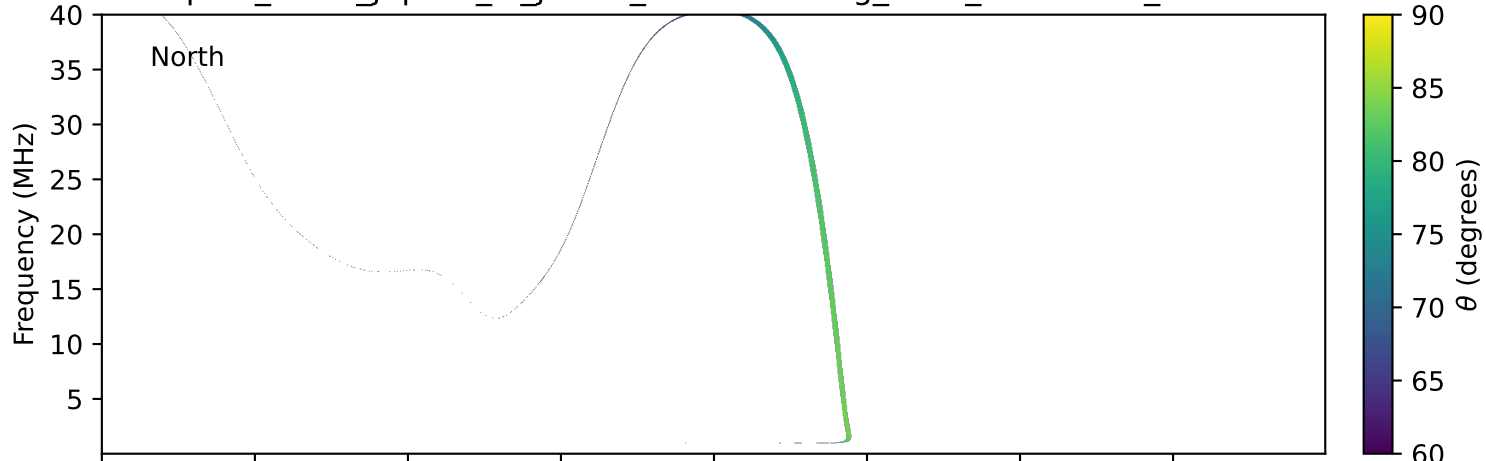
expres_earth_jupiter_io_jrm33_lossc-wid1deg_3kev_20230327_v11.cdf
