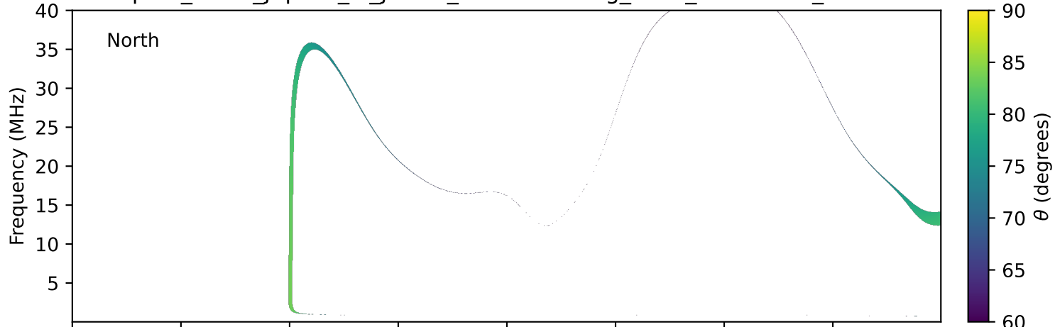
expres_earth_jupiter_io_jrm33_lossc-wid1deg_3kev_20230323_v11.cdf
