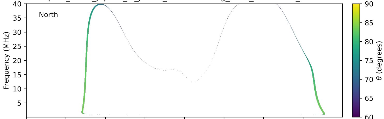
expres_earth_jupiter_io_jrm33_lossc-wid1deg_3kev_20230316_v11.cdf
