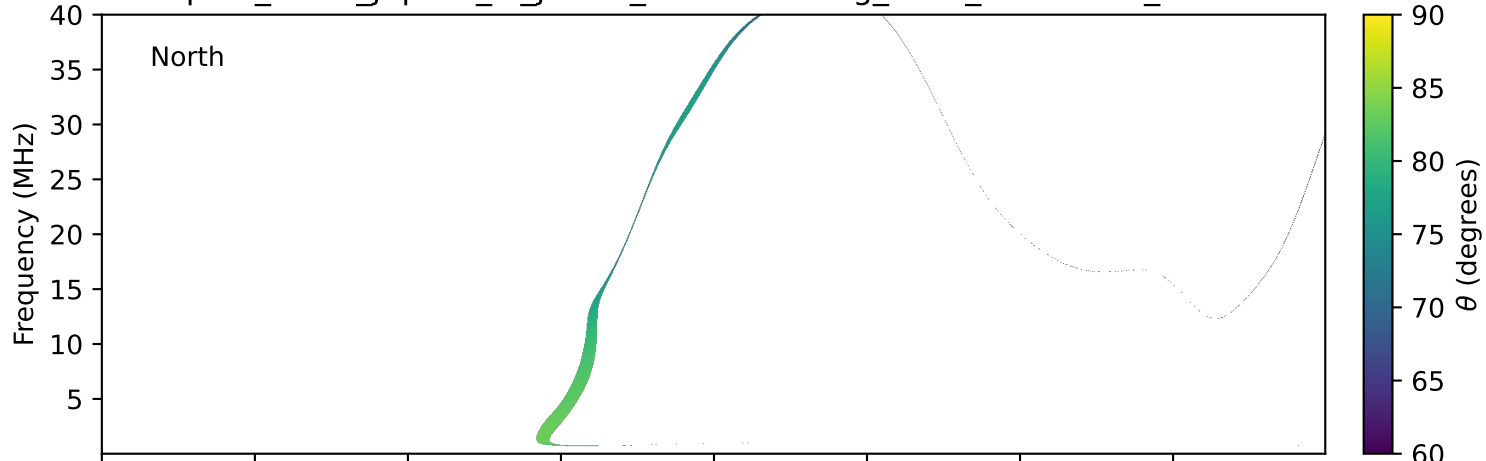
expres_earth_jupiter_io_jrm33_lossc-wid1deg_3kev_20230314_v11.cdf
