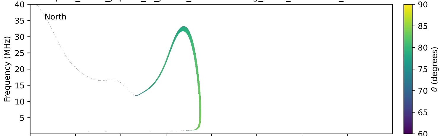
expres_earth_jupiter_io_jrm33_lossc-wid1deg_3kev_20230313_v11.cdf
