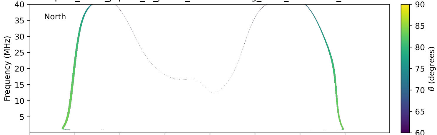
expres_earth_jupiter_io_jrm33_lossc-wid1deg_3kev_20230309_v11.cdf
