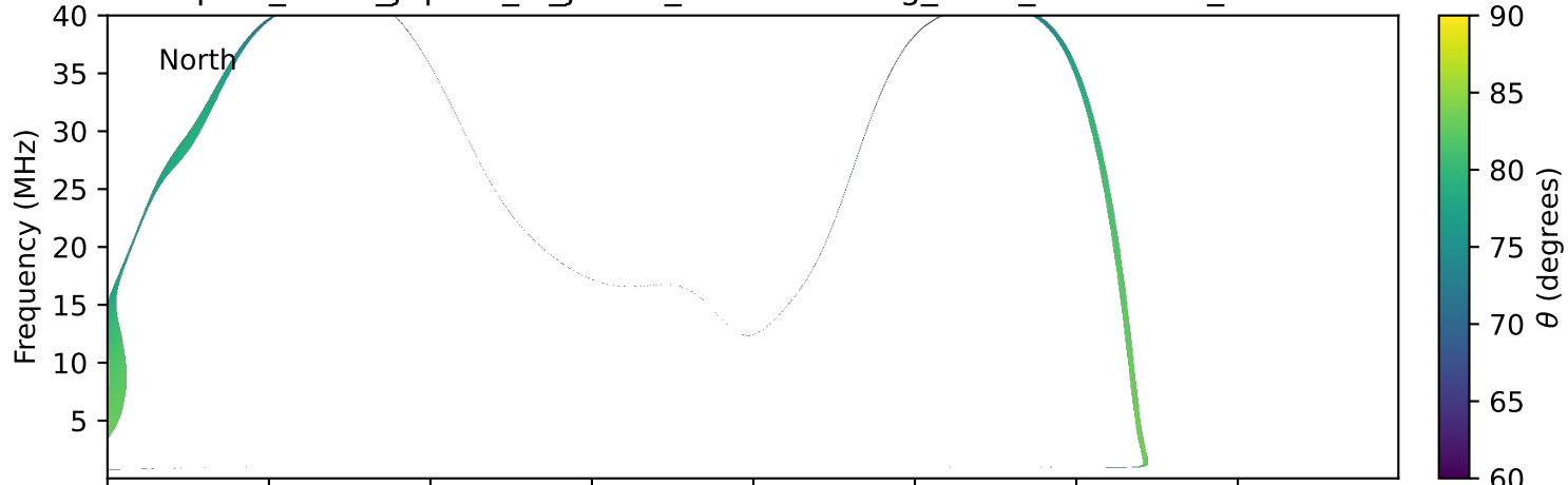
expres_earth_jupiter_io_jrm33_lossc-wid1deg_3kev_20230302_v11.cdf
