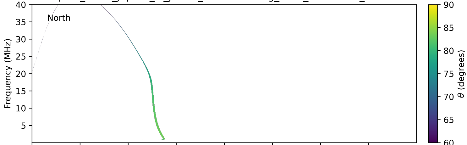
expres_earth_jupiter_io_jrm09_lossc-wid1deg_3kev_20230329_v11.cdf
