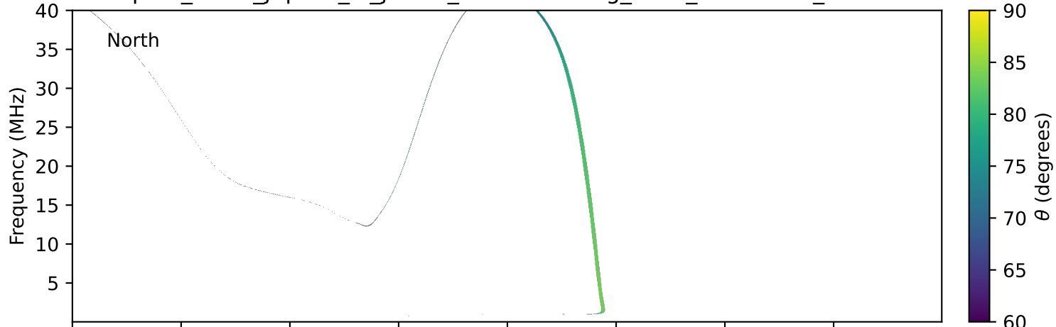
expres_earth_jupiter_io_jrm09_lossc-wid1deg_3kev_20230327_v11.cdf
