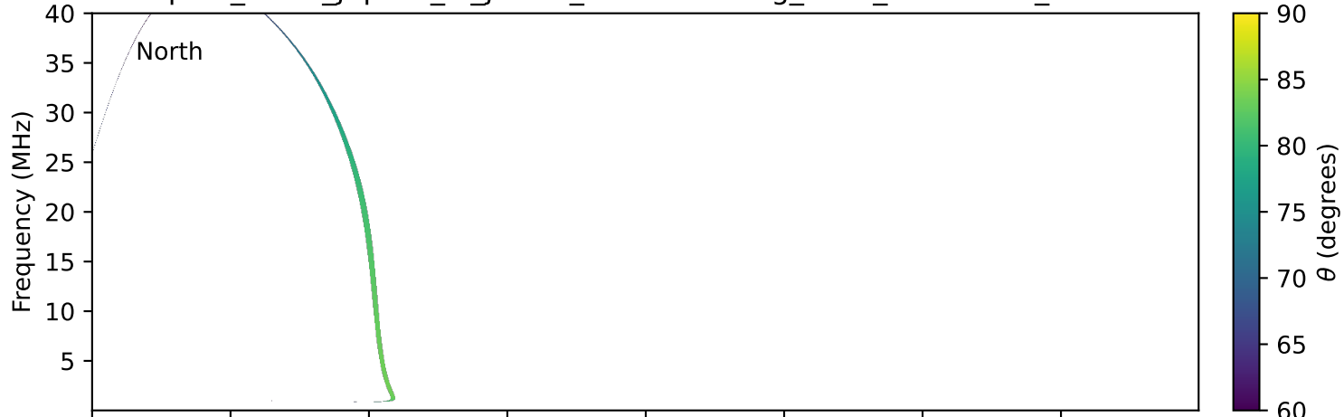
expres_earth_jupiter_io_jrm09_lossc-wid1deg_3kev_20230322_v11.cdf
