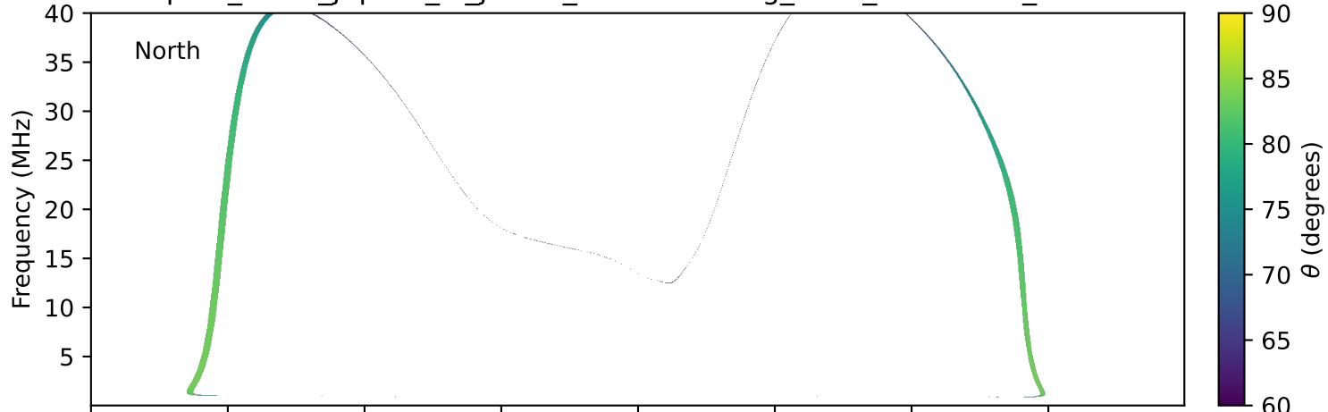
expres_earth_jupiter_io_jrm09_lossc-wid1deg_3kev_20230309_v11.cdf
