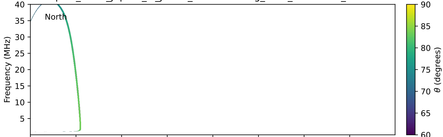
expres_earth_jupiter_io_jrm09_lossc-wid1deg_3kev_20230308_v11.cdf
