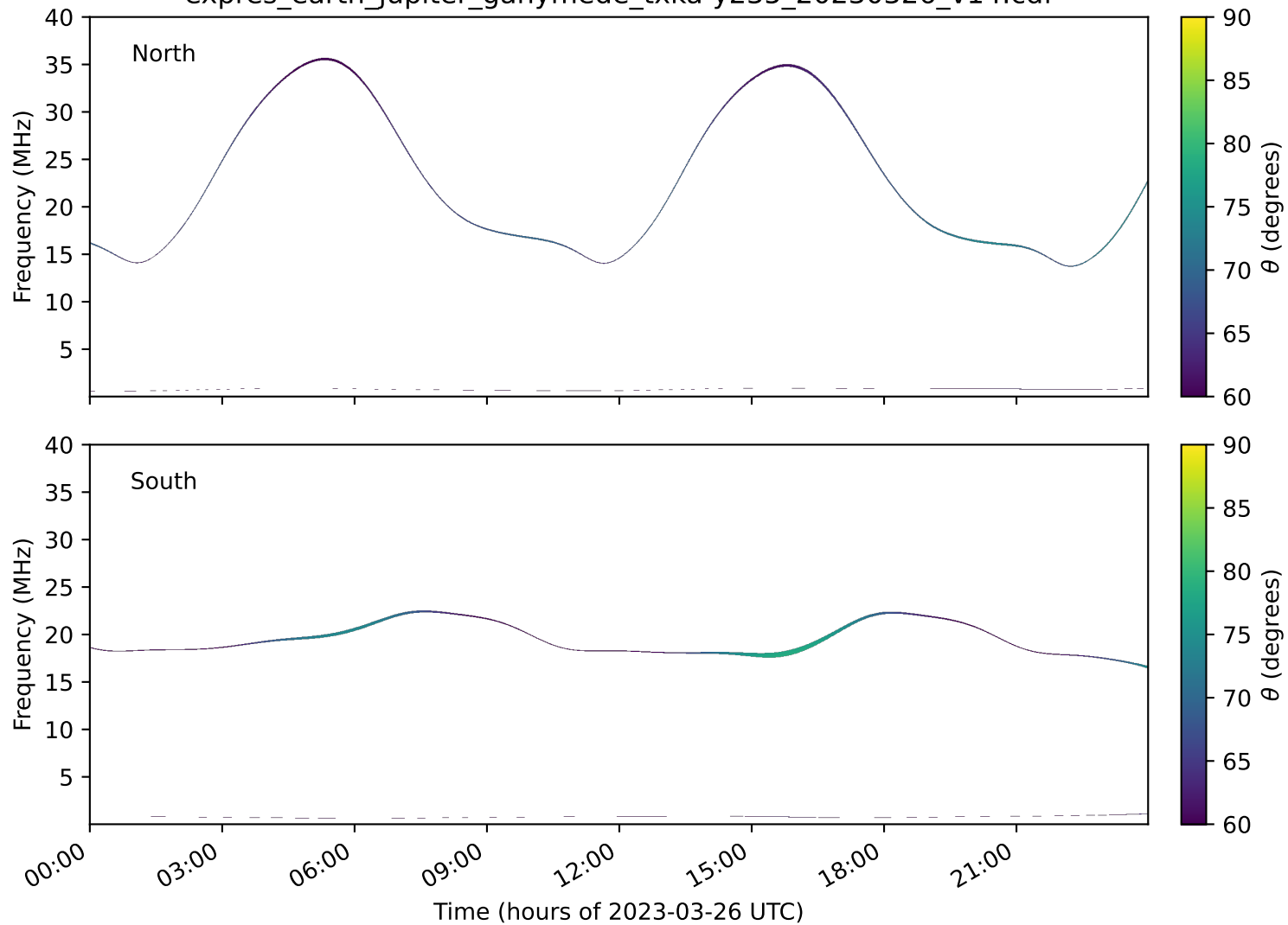
expres_earth_jupiter_ganymede_txka-y235_20230326_v14.cdf
