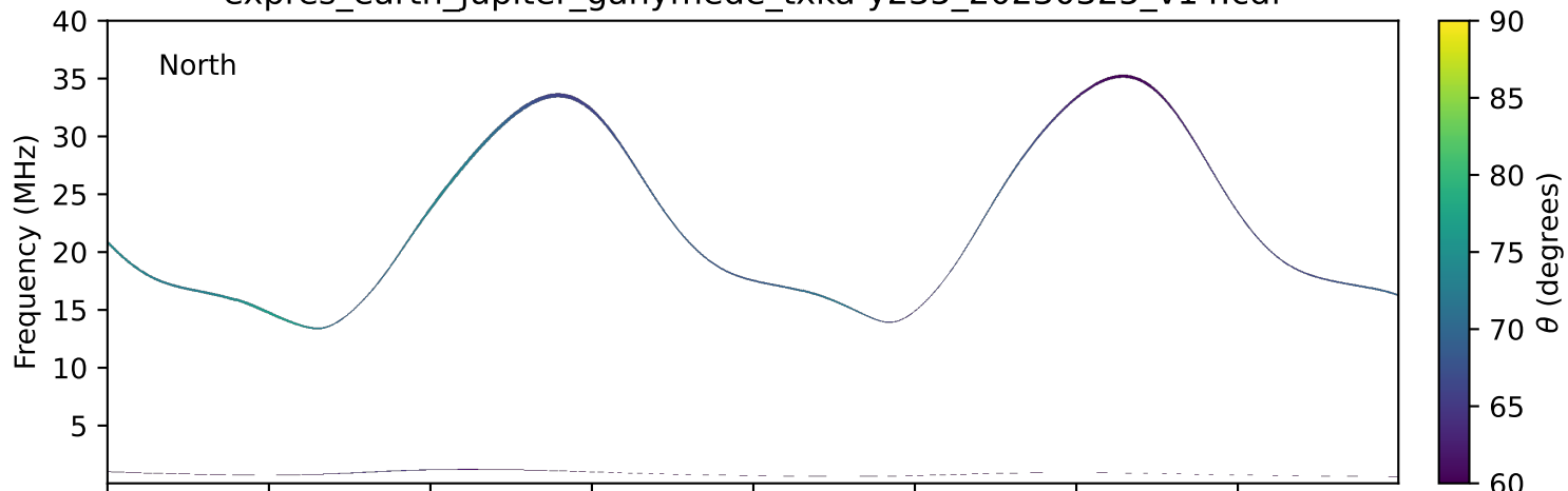
expres_earth_jupiter_ganymede_txka-y235_20230325_v14.cdf
