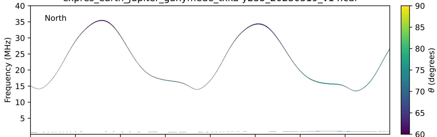
expres_earth_jupiter_ganymede_txka-y235_20230319_v14.cdf
