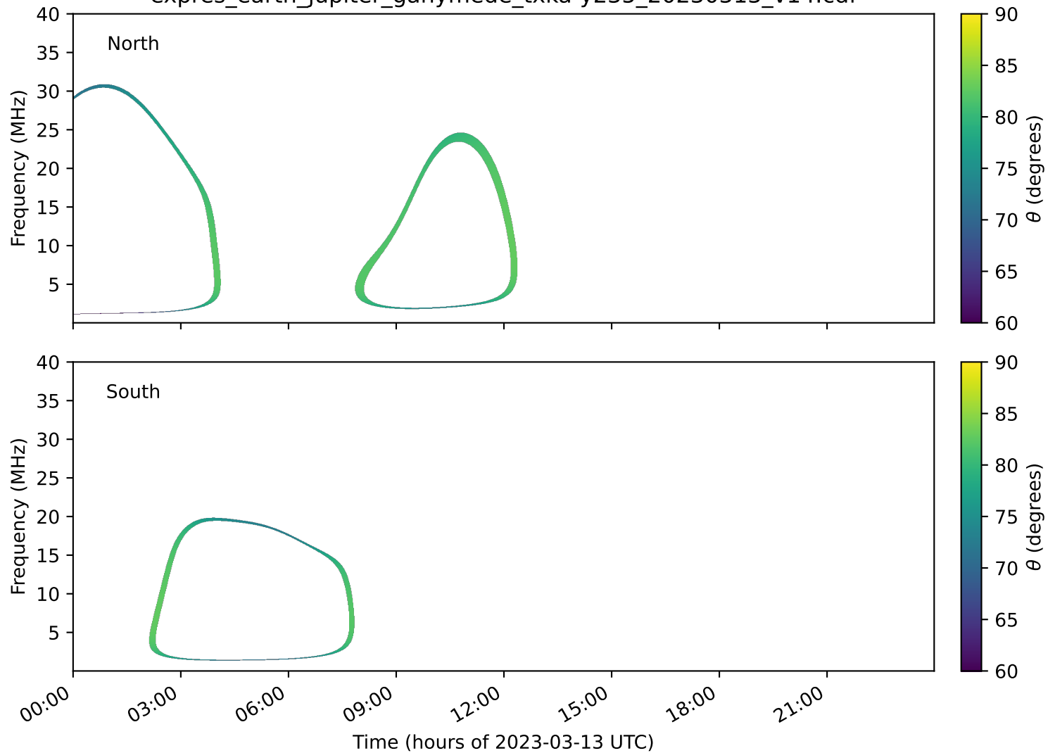
expres_earth_jupiter_ganymede_txka-y235_20230313_v14.cdf
