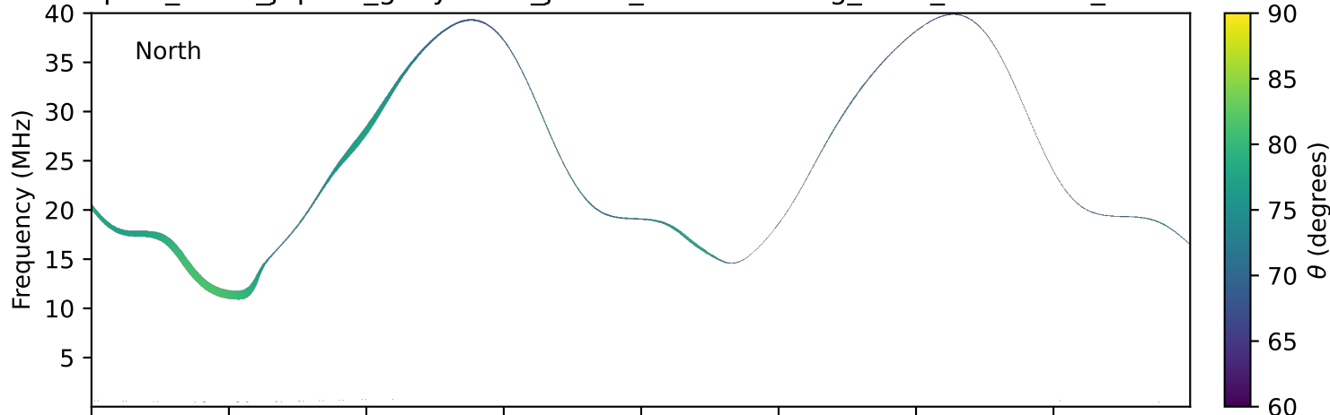
expres_earth_jupiter_ganymede_jrm33_lossc-wid1deg_3kev_20230325_v11.cdf
