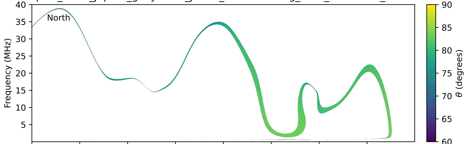
expres_earth_jupiter_ganymede_jrm33_lossc-wid1deg_3kev_20230320_v11.cdf
