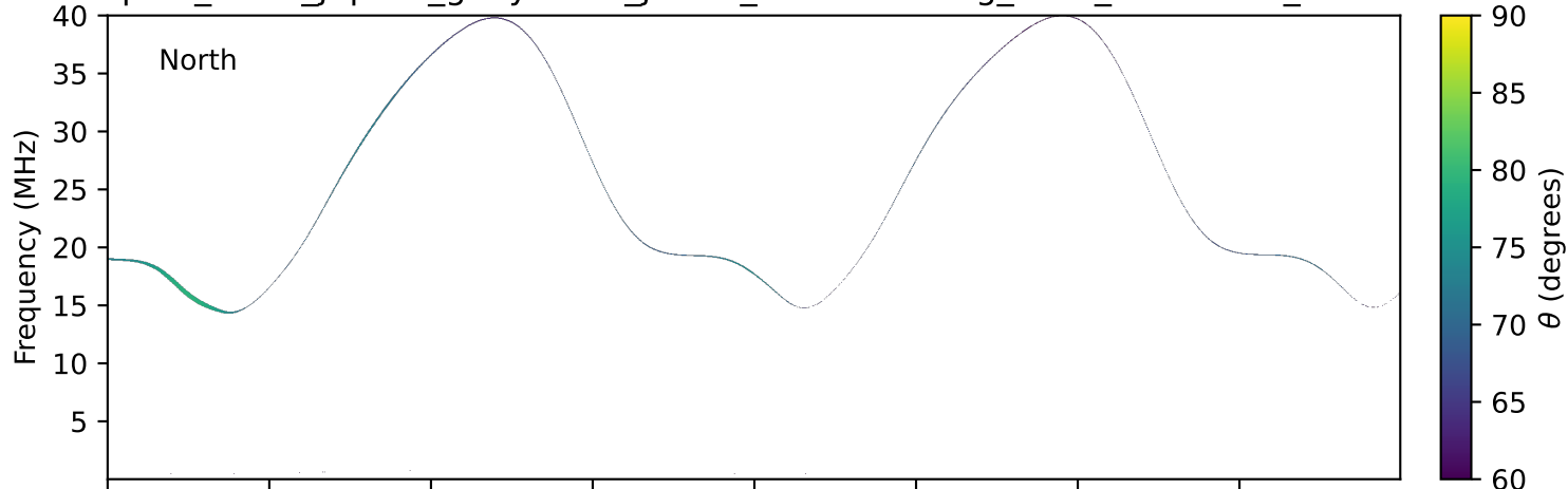
expres_earth_jupiter_ganymede_jrm33_lossc-wid1deg_3kev_20230311_v11.cdf
