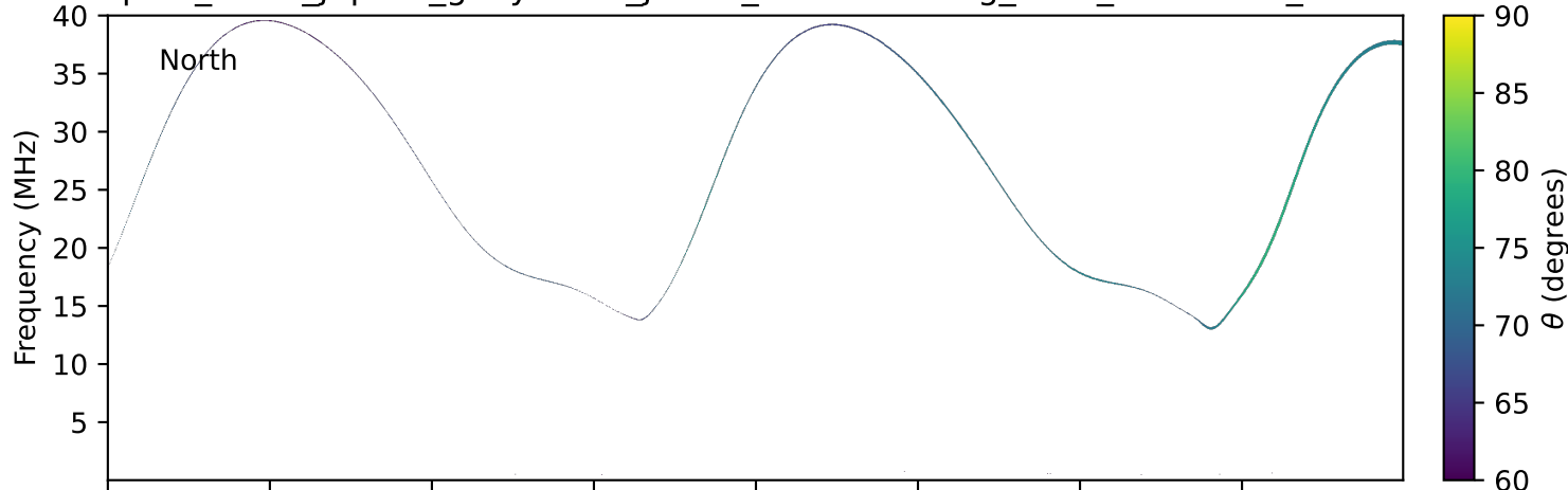
expres_earth_jupiter_ganymede_jrm09_lossc-wid1deg_3kev_20230305_v11.cdf
