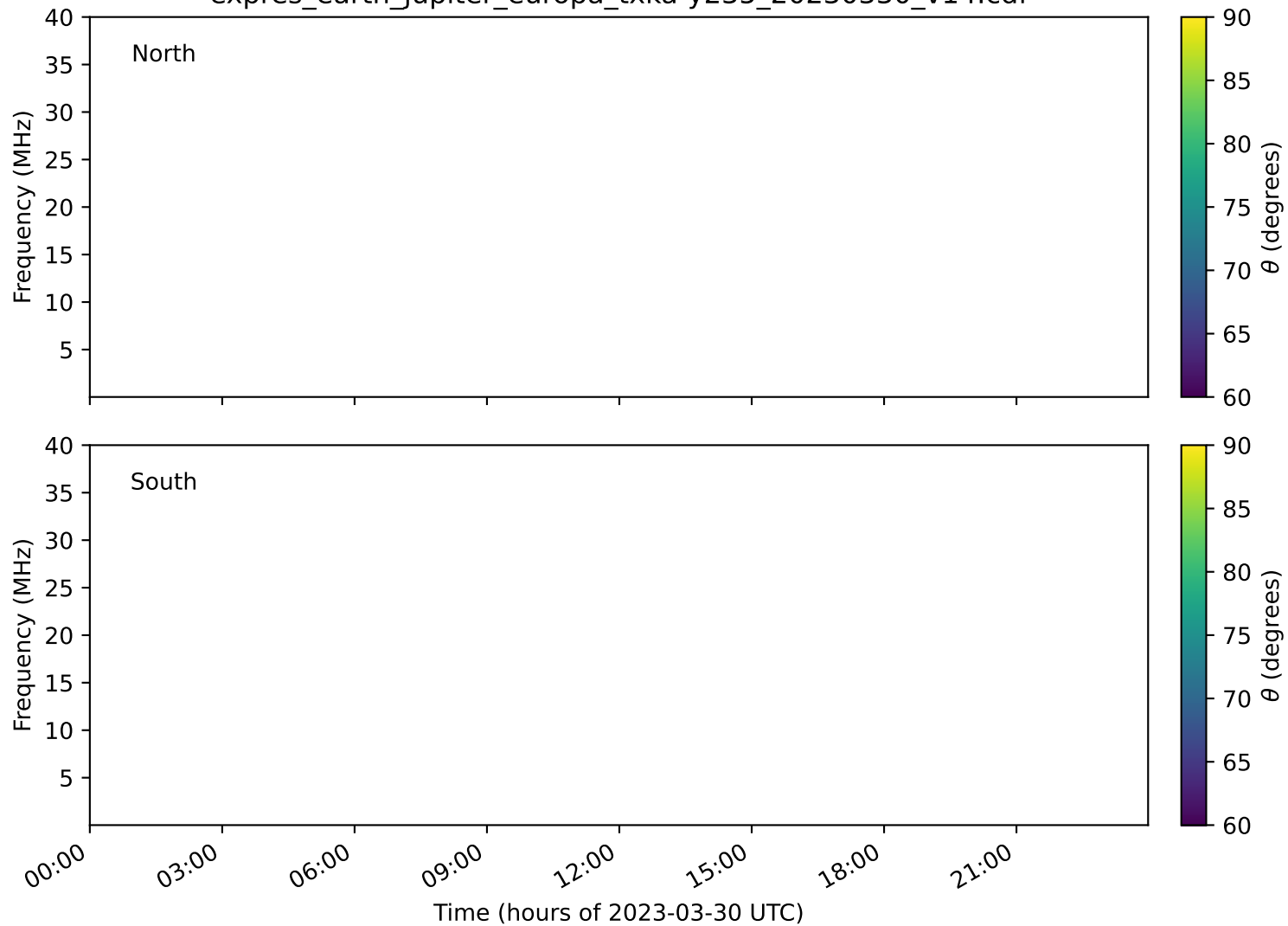
expres_earth_jupiter_europa_txka-y235_20230330_v14.cdf
